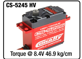
CS-5245 HV Ultra High Torque - HV - Coreless - Steel Gears - Ball Beared Torque @ 8.4V 46.9 kg/cm
